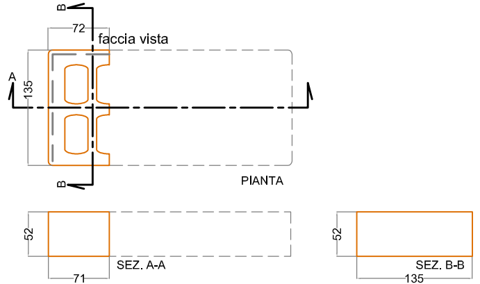
MATTONE 1/4
