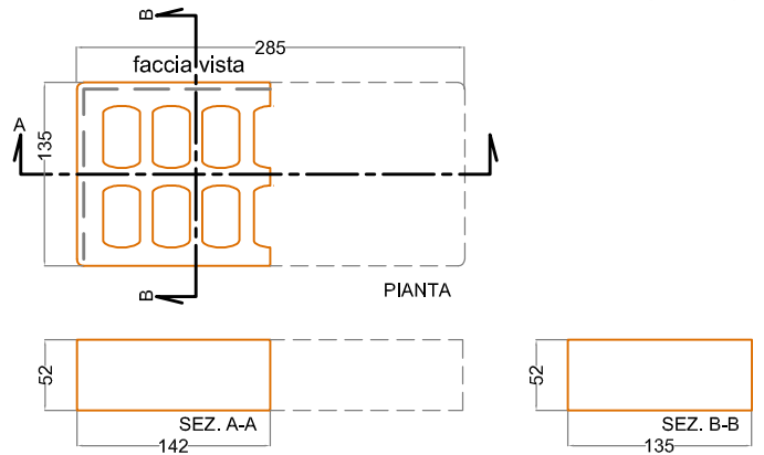
MATTONE 1/2
