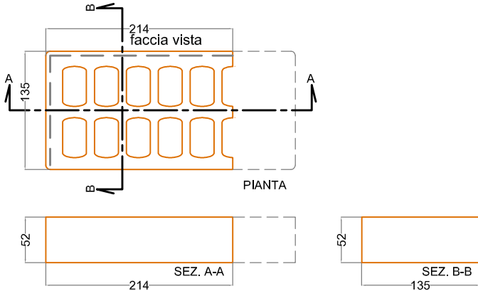
MATTONE 3/4
