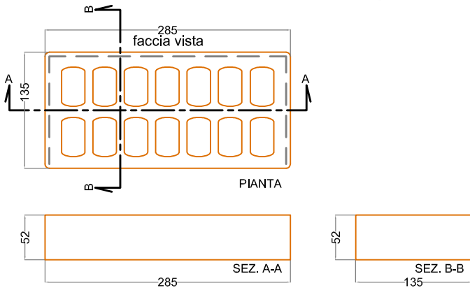
MATTONE INTERO
